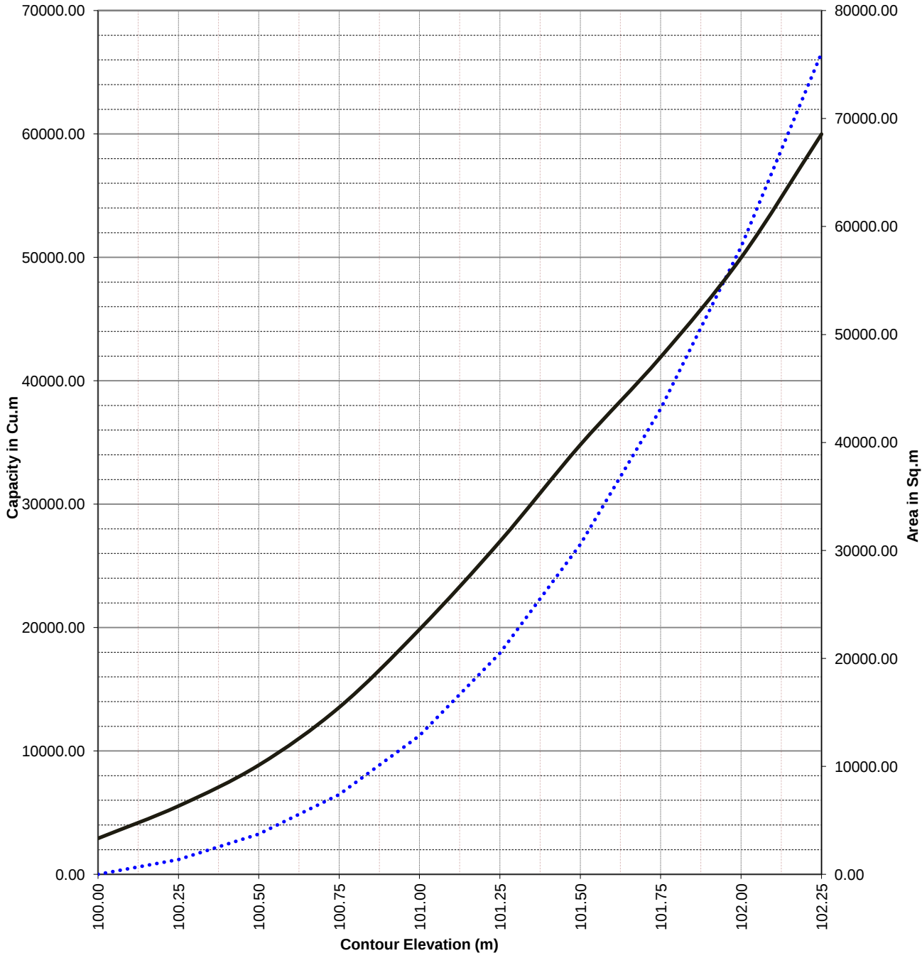
Area Capacity Diagram Kuda Kadiyawa Wewa
