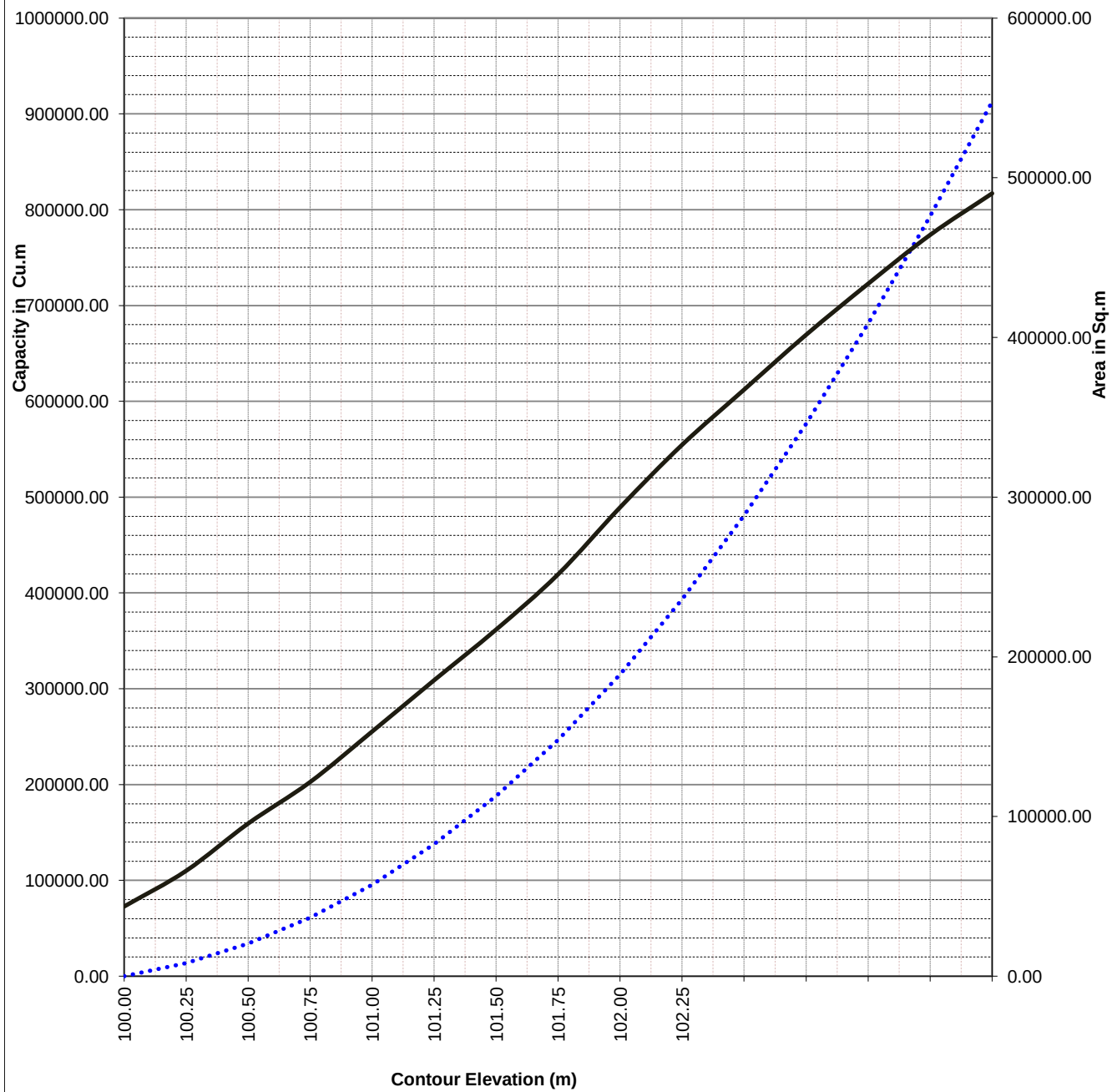
Area Capacity Diagram Galkadawala Maha Wewa
